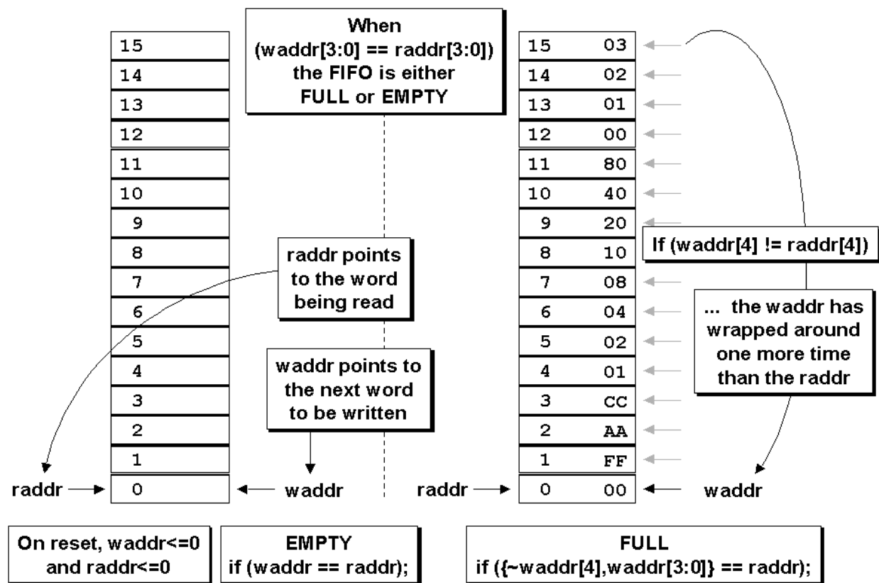
Figure 1 - FIFO full and empty conditions (using binary pointers)
